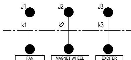
Torsional rigidity [Nm/rad] (kg.m²) k1 k2 k3 J1 J2 J3 1.79 E+7 3.79 E+7 1.60 E+7 7.8 31.1 1.5 1.79 E+7 3.68 E+7 1.68 E+7 7.8 34.7 1.5 1.79 E+7 3.54 E+7 1.51 E+7 7.8 40 1.6 1.79 E+7 3.36 E+7 1.67 E+7 7.8 47.2 1.5 1.79 E+7 3.13 E+7 1.32 E+7 7.8 57.5 1.3
